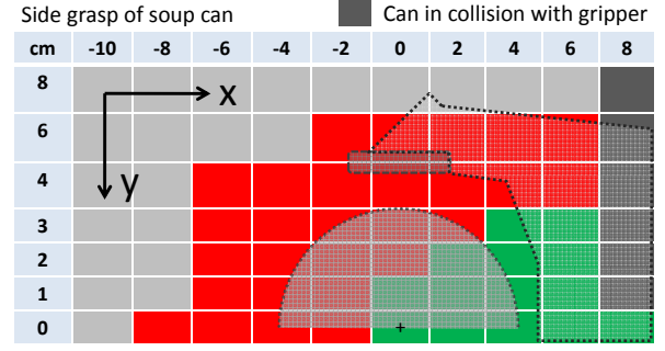
Fig. 7. Reactive vs. open-loop grasping for side grasps, under a wide range of positioning errors.
