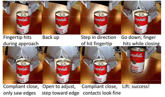
Fig. 5. Example of a reactive grasp sequence using the complete set of reactive adjustments.
