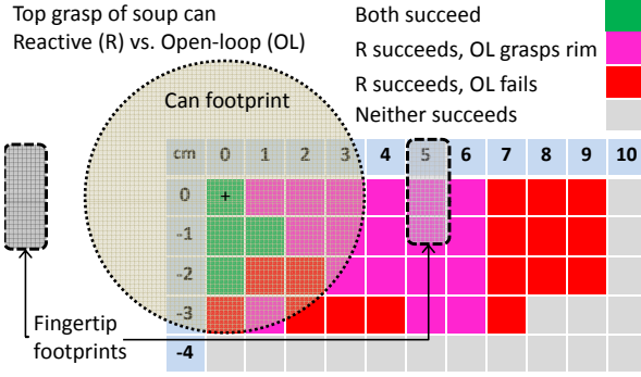
Fig. 6. Reactive vs. open-loop grasping for overhead grasps, under a wide range of positioning errors.
